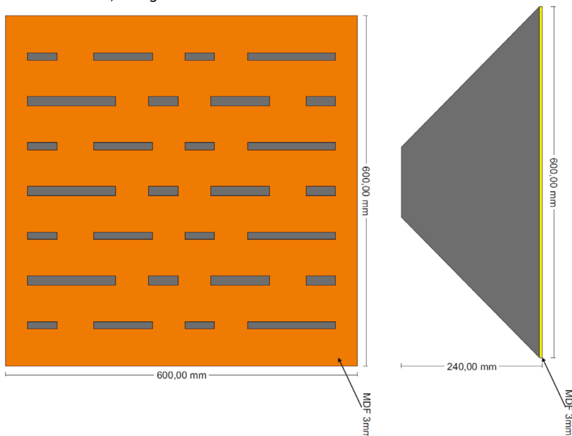
Picture 1: schematic drawing of the Decotrap sound-absorption cladding.
