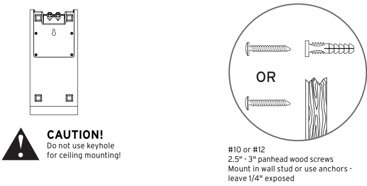
FIGURE 4 WALL MOUNTING SURROUND SPEAKERS
