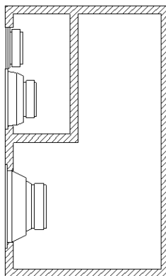
Sealed cabinet
