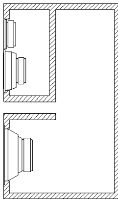
Bass reflex cabinet
