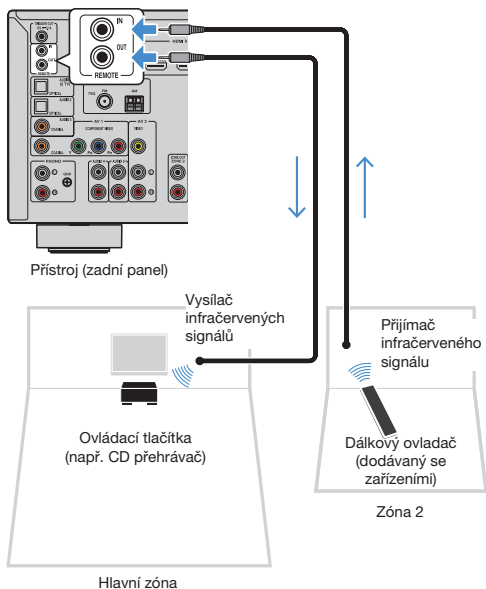
Konektory REMOTE IN/OUT
