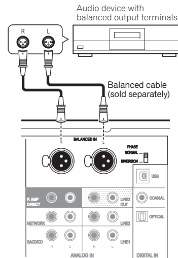
A-70DA's rear panel
