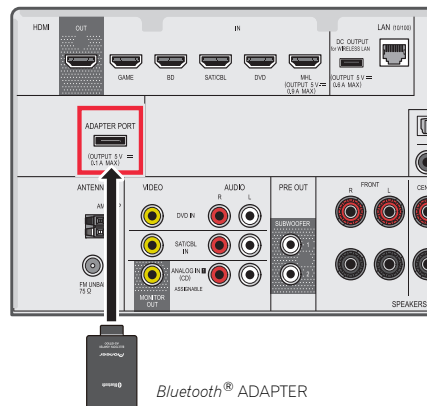
Bluetooth ® ADAPTER
