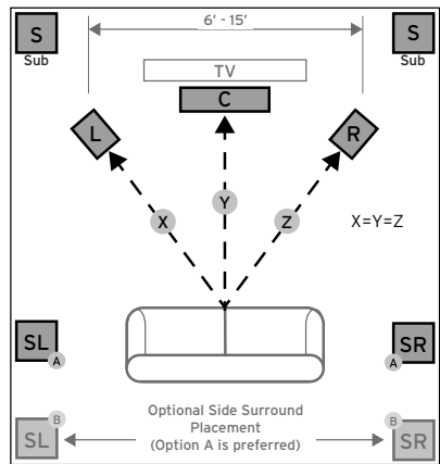
FIGURE 1 SPEAKER PLACEMENT IN LISTENING AREA
